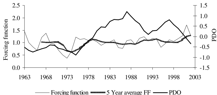
Figure 27. Forcing function and five year running average of the forcing function (FF) estimated to fit the 1963 model to time series data and for comparison the 5 year running average of the Pacific Decadal Oscillation (PDO).
