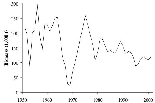
Figure 7. Biomass time series of herring in the BC shelf ecosystem. This represents a composite of 5 stocks that form the majority of herring in the area (Anonymous 2002a,b,c,d,e).
