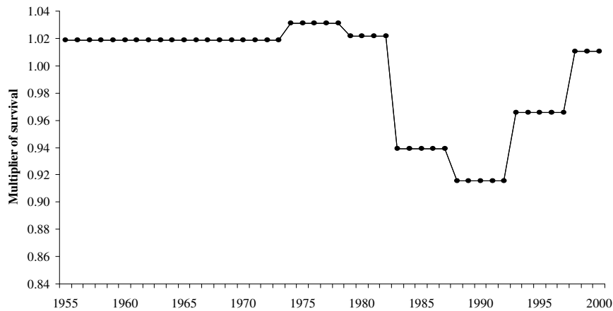
Figure 4. Multiplier of survival used on both adult and pups of Steller sea lions.
