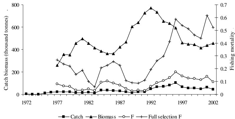
Figure 12. Catch (10 3 tonnes), biomass (10 3 tonnes) and fishing mortality (F, year -1 ) for Atka mackerel in the Aleutian Islands. F is catch/(age 1+ biomass); the full selection F is the annual fishing mortality of fish fully selected by the fishing gear.
