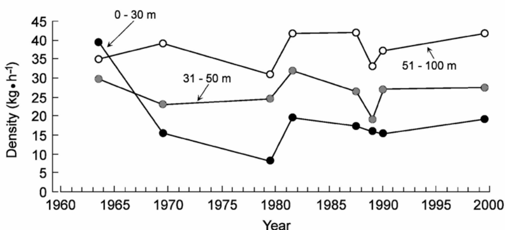
FIG. 3. — Apparent abundance of demersal resources on the shelf of Ghana, as estimated from successive bottom trawl surveys, 1963-2000. Note that the cod end mesh size in 2000 was half that in earlier survey, resulting in an overestimate of density for that year (see text).
