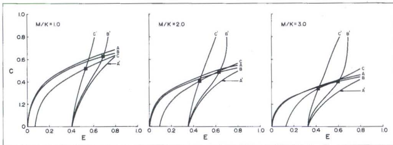
Fig. 4. Change in position of eumetric fishing lines in the E, C plane with increasing selection range ( \Delta C ). The lines marked A, B and C indicate the location of optimum C's at fixed E, while the lines marked A', B' and C' indicate the location of optimum E's at fixed C values. The \Delta C values are 0 for A and A', 0.02 for B and B' and 0.10 for C and C'. See text.
