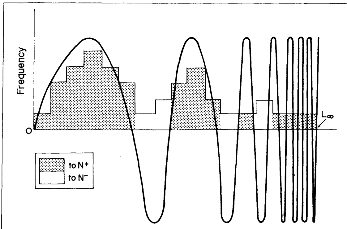
Fig. 2. The SLCA method estimates L_{\infty} and K by reexpressing the VBGF as an oscillating line whose limit is ( L_{\infty} ) and whose frequency of oscillation is determined by K . The frequencies comprised between the positive parts of oscillations are multiplied with the value of the corresponding section of the oscillatory curve, then added to a positive counter ( N+ ); while the corresponding products for the negative parts are added to a negative counter ( N- ). The scoring function is then S = N++ N- . The problem is that the number of cohorts represented by each length class is not taken into account. This can be achieved, however, by division of each frequency by the corresponding \Delta t value.
