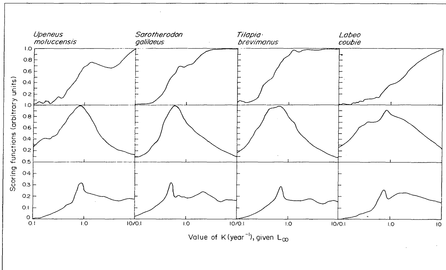
Fig. 3. Four examples of the differences and similarities between the old version of SLCA (top row), the new version of SLCA (NSLCA; middle row), and the ELEFAN I routine (bottom row). [Files other than MUMORG are from Moreau et al. 1995].
