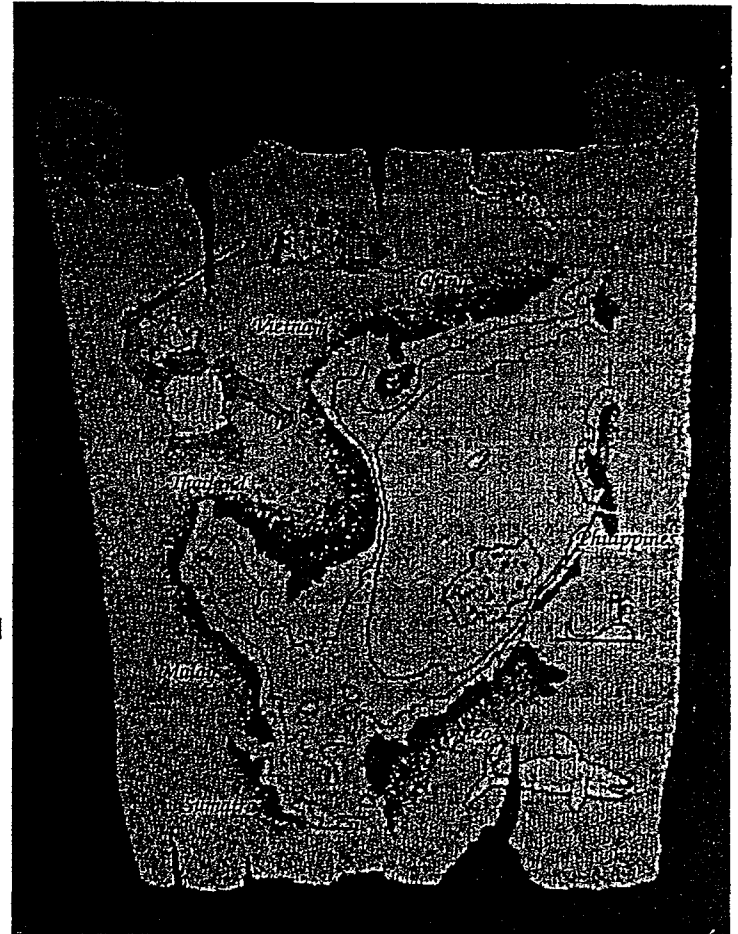
Fig. 1. The South China Sea as defined in this contribution covers 3.5 million km 2 of mainly shallow waters (< 200 m).
