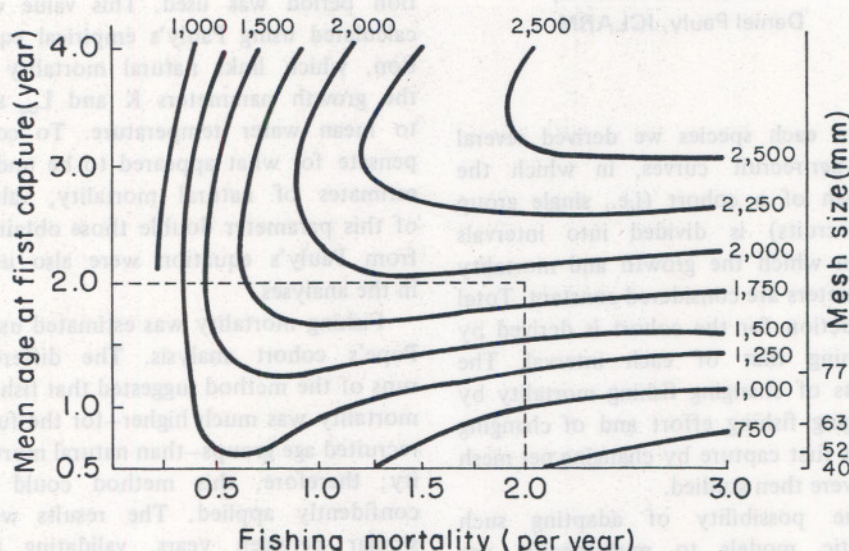
Fig. 1. Yield (in tonnes) for Pseudotolithus senegalensis as a function of fishing mortality and mean age at first capture and M = 0.15 . For example, if fish become catchable at age 2 years and fishing mortality is estimated at 2.0, the expected yield is between 1,750 and 2,000 t.
