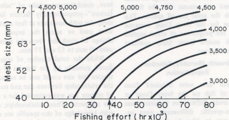
Fig. 2. Yield (in tonnes) as related to mesh size and fishing effort on the seven major trawl species of the Ivory Coast. The arrow shows the present effort level.
